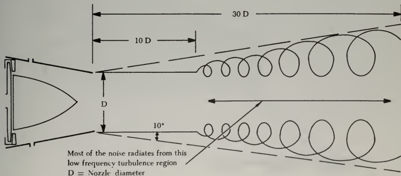
FIGURE 2-40. Turbojet exhaust noise pattern.
